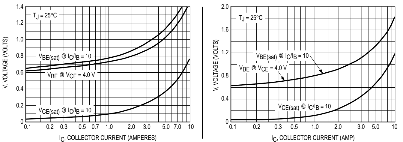
Figure 5. "On" Voltages
