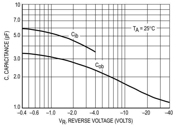
Figure 4. Capacitance
