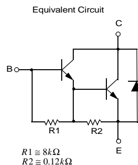
TO-3P 1.Base 2.Collector 3.Emmitter
