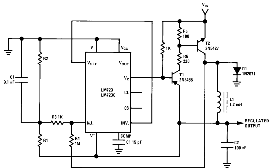
FIGURE 9. Positive Switching Regulator
