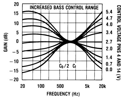
FIGURE 5. Tone Characteristic (Gain vs Frequency)
