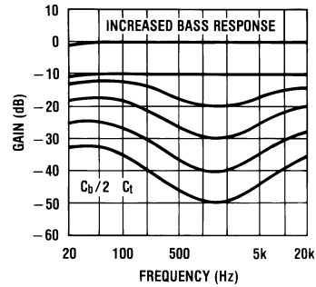
FIGURE 8. Loudness Compensated Volume Characteristic
