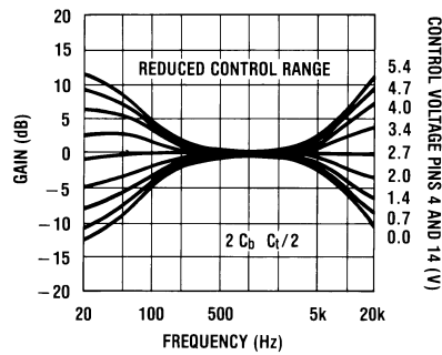
FIGURE 4. Tone Characteristic (Gain vs Frequency)
