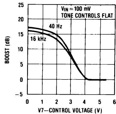
Loudness Control Characteristic
