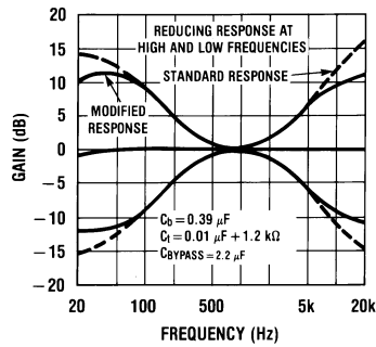
FIGURE 6. Tone Characteristic (Gain vs Frequency)
