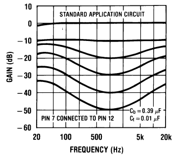
FIGURE 7. Loudness Compensated Volume Characteristic
