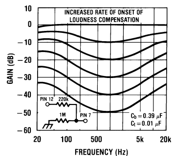
FIGURE 12. Loudness Compensated Volume Characteristic
