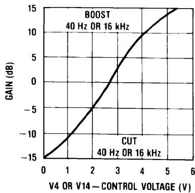
Tone Control Characteristic
