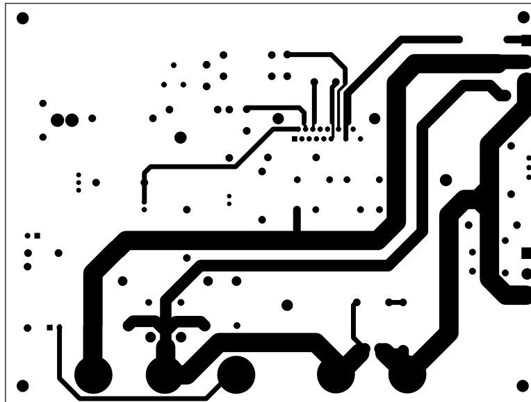
Figure 8. Bottom Layer
