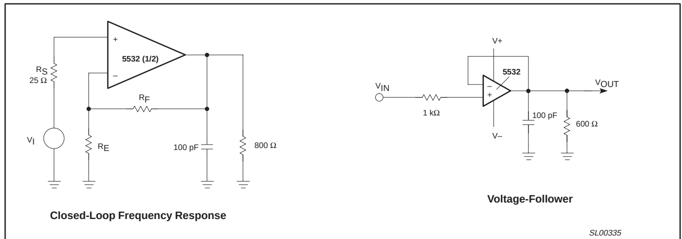
Figure 4. Test Circuits
