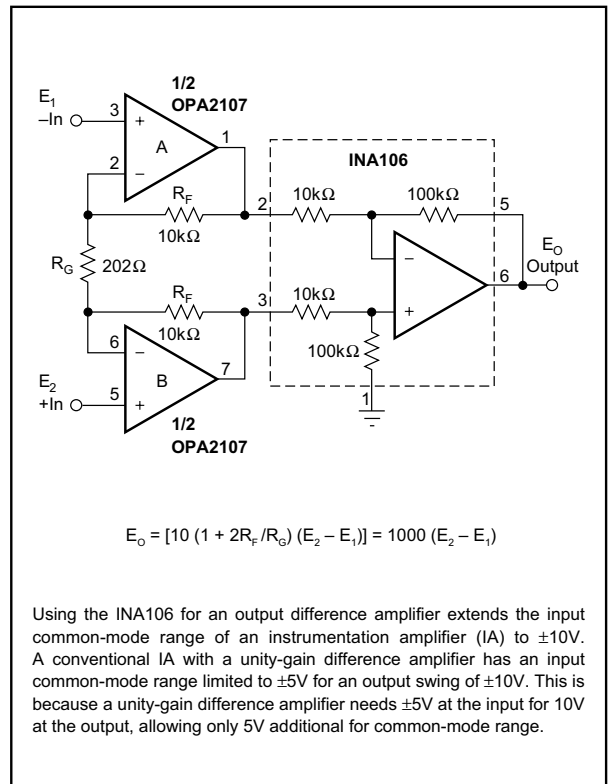
FIGURE 3. Precision Instrumentation Amplifier.
