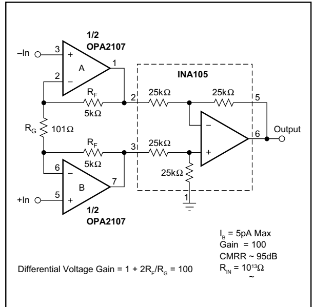
FIGURE 2. FET Input Instrumentation Amplifier.
