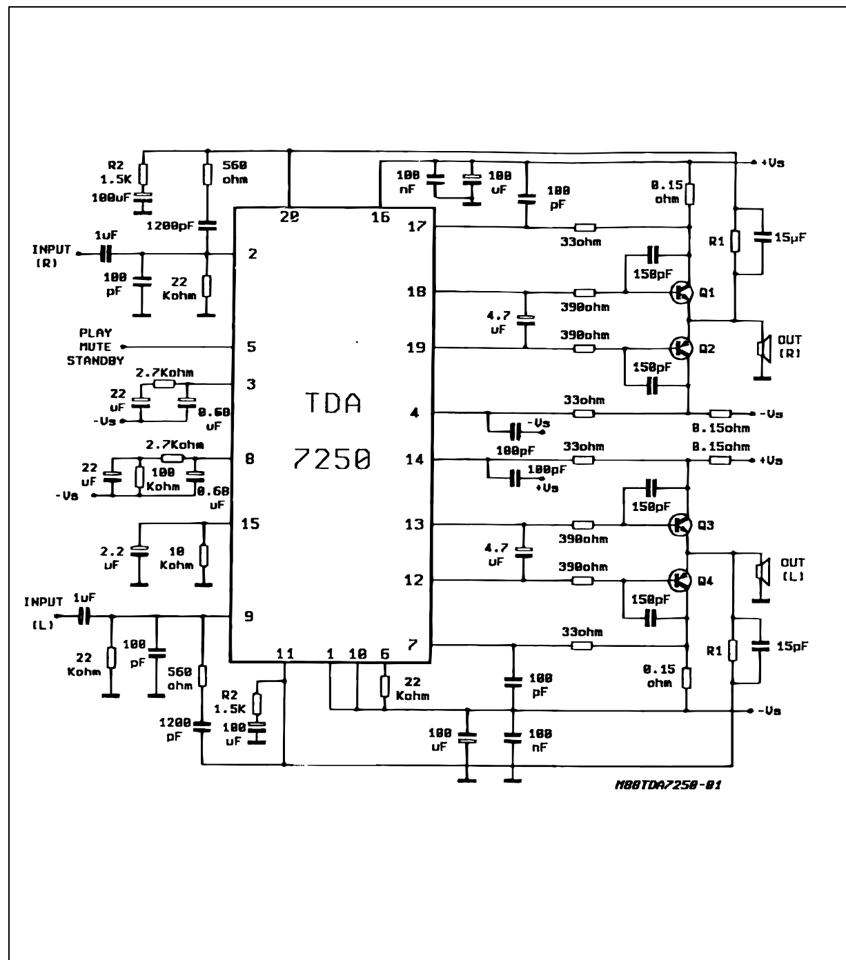
Note : Q1/Q2 = Q3/Q4 = \text{TIP } 142/\text{TIP}147 GV = 1 + R1/R2
